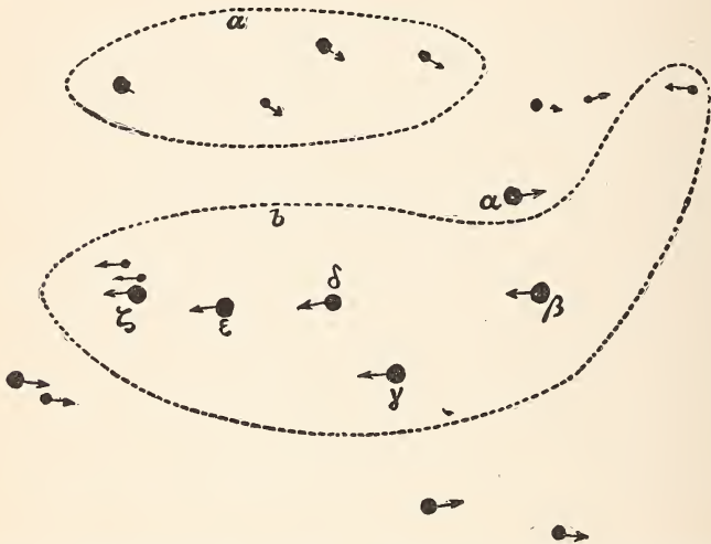
FIG. 11.—OBSERVED PROPER MOTIONS OF STARS IN URSA MAJOR AND NEIGHBORHOOD.
